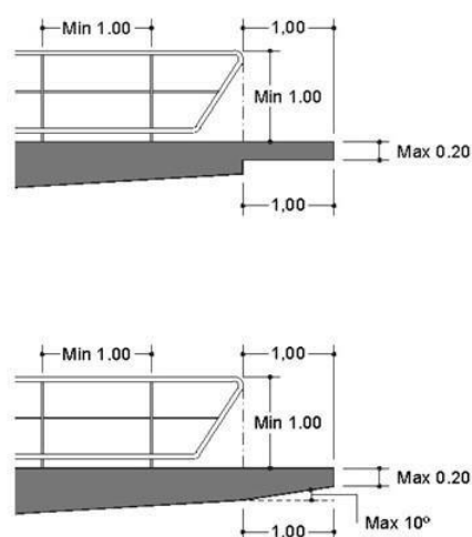
Handrail and Platform Front Edge Detail
